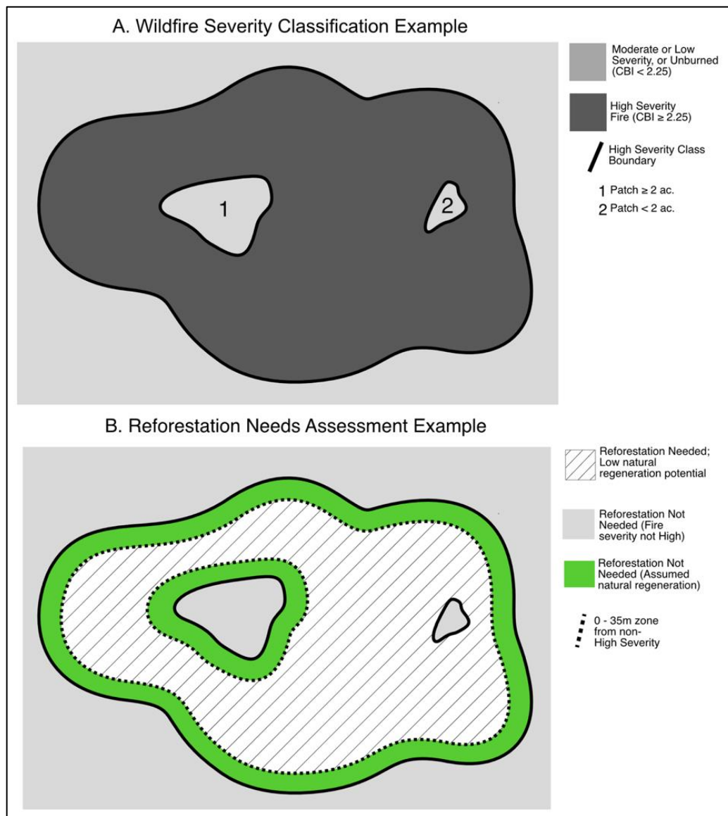
Figure 1. Identifying reforestation needs from wildfire spatial data
